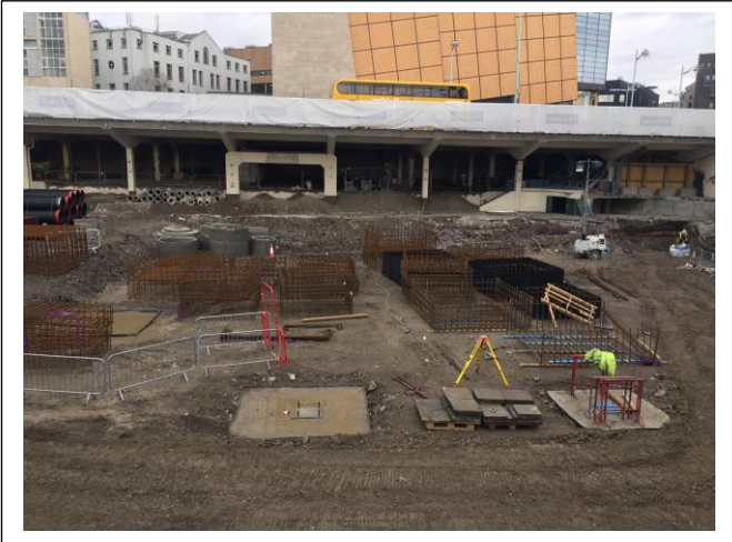
Reinforcement for foundations being pre-fabricated.
